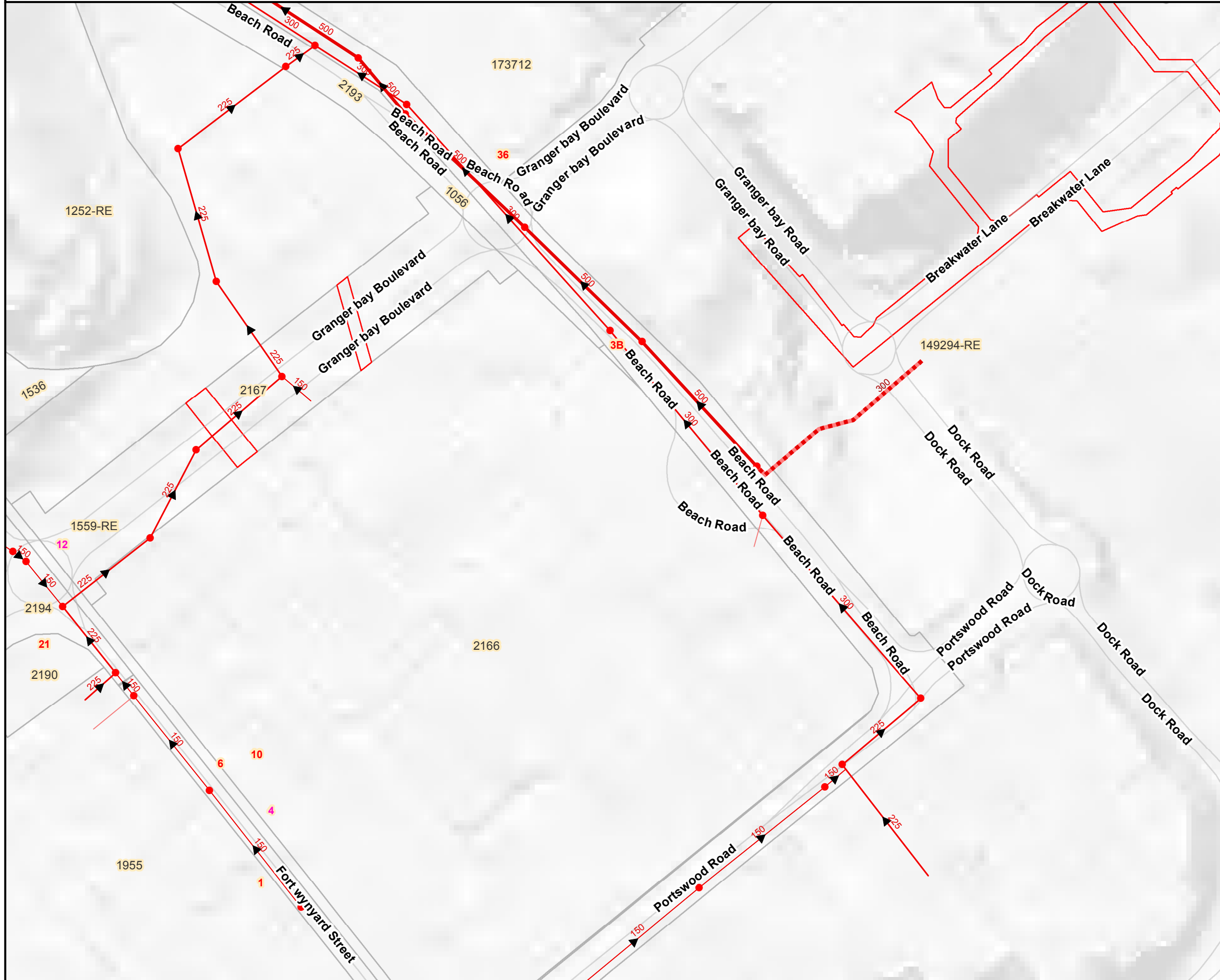
Figure 2 - Existing Sewer Conveyance Network
